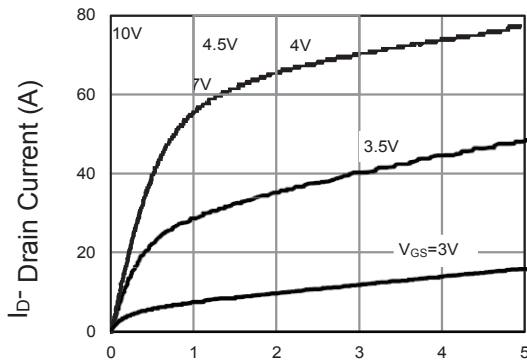
Vds Drain-Source Voltage (V) Figure 1 Output Characteristics
